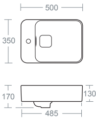
FUSARO 50CM RECTANGULAR VESSEL BASIN WITH SIDE TAP DECK
